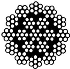
19 x 7 ROTATION RESISTANT WITH WIRE STRAND CORE
