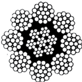
8 x 25 ROTATION RESISTANT WITH IWRC
